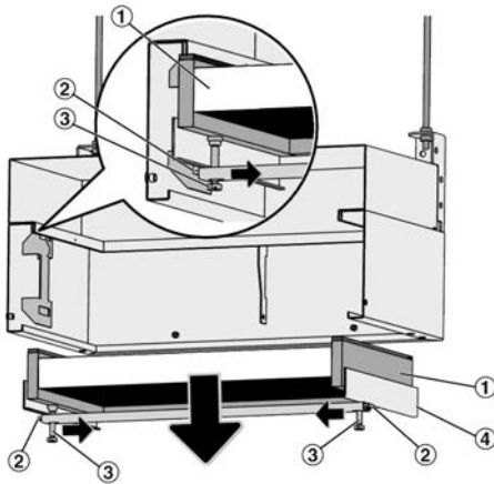
Fig. 11: Filter change
